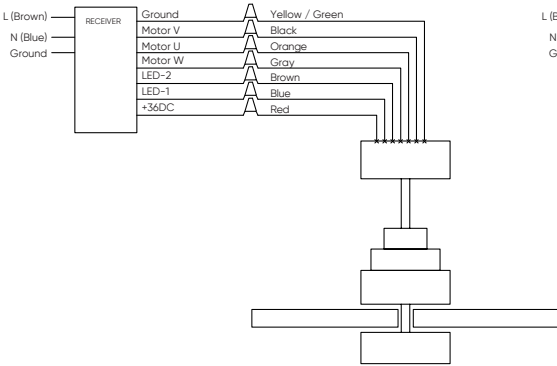
SUPPLY CIRCUIT
