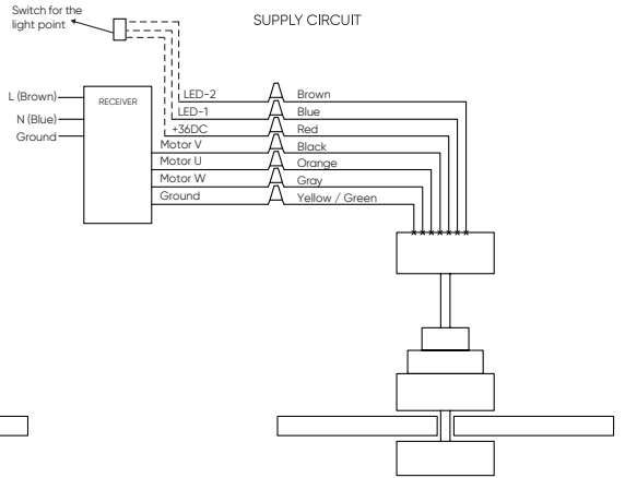
SUPPLY CIRCUIT
